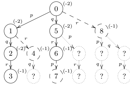
Fig. 1. Left: Code of working example (up) and ICs (down). Right: Execution tree starting from z = -2, x = -2 . Full tree computed by SDPOR, dotted fragment not computed by SDPOR, and, dashed+dotted fragment not computed by CDPOR.
